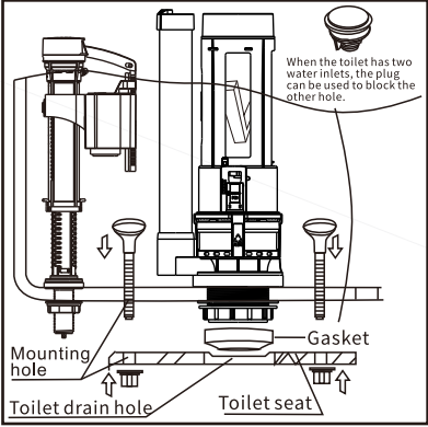
Split toilet installation method
