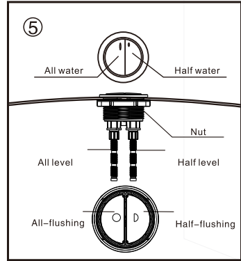
adjust the button to make the halt level aim at Half water button, all level aim at all water button, rotate nut and lock it.
