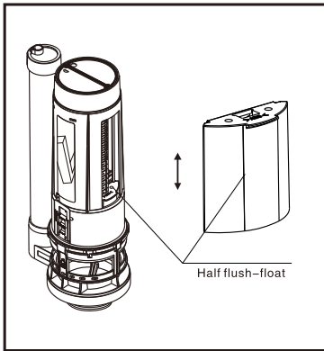
Adjust half key float to control its displacement, float is higher, its displacement will be less.
