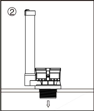
Install the base into drainer hole, adjust it perfectly to the wall if water tank, rotate it with suitable angles.
