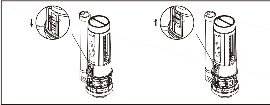
Adjust the all water controller to control its water volume, when turn it down, the button hole will close, its water volum, will be more, and vice versa.
