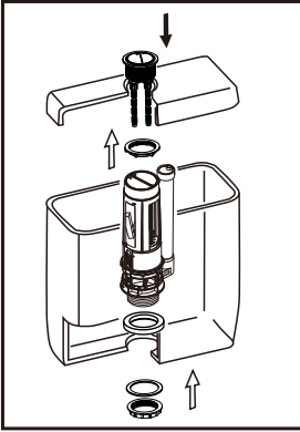
Screw-in, two-piece
