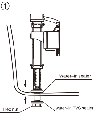
Take off the Hex nut, and put the Fill valve in to the hole, adjust the body position. lock the Hex nut .
