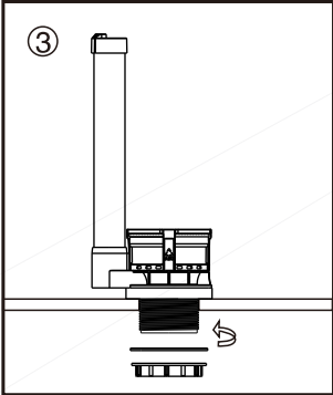
lock it with plastic screw, make the seal ring completely with tank draining hole, then install the valve.
