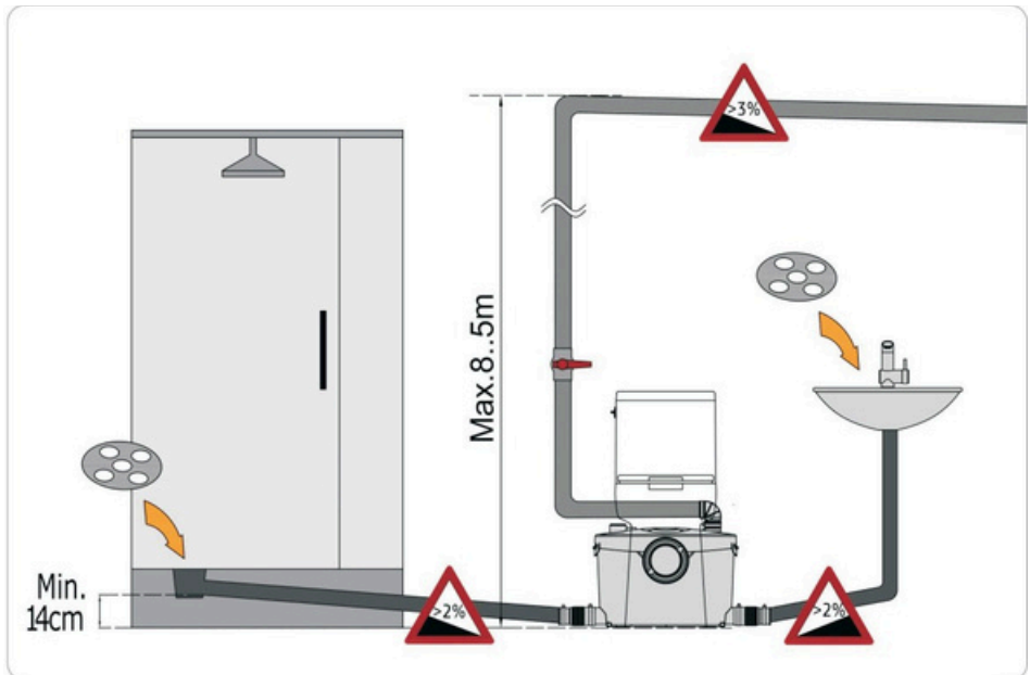
Fig4: Connection
