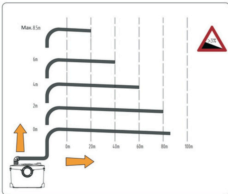
Fig10: Pumping head
