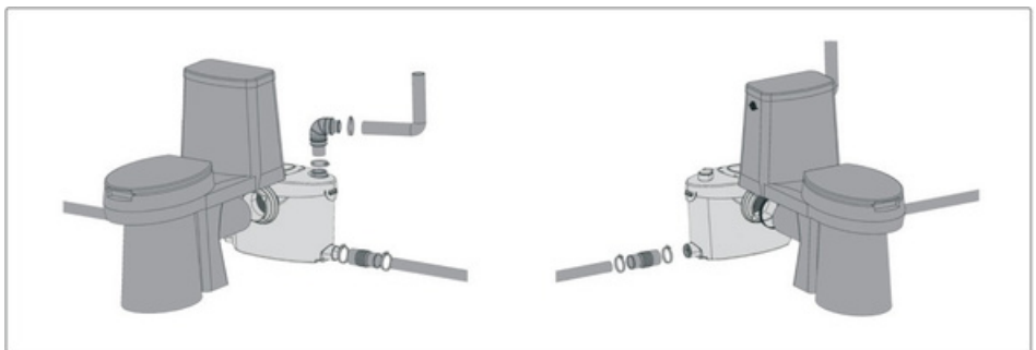
Fig4: Connection
