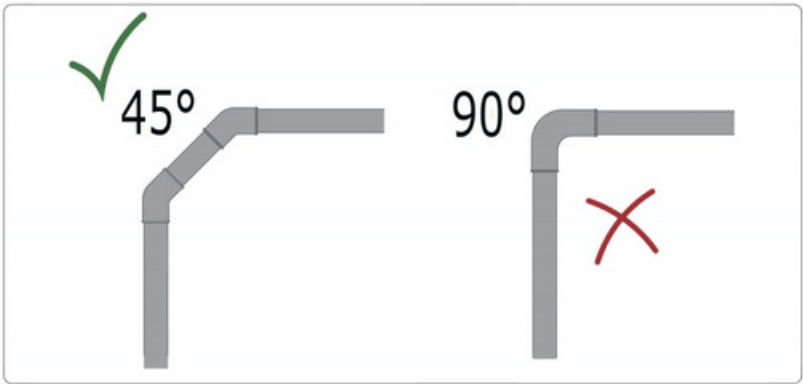
Fig14&15: Discharge pipe connection
