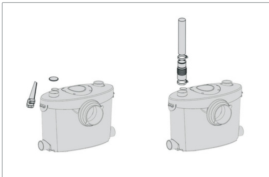
Fig6: Inlet cover (Cover the inlets for unused)
