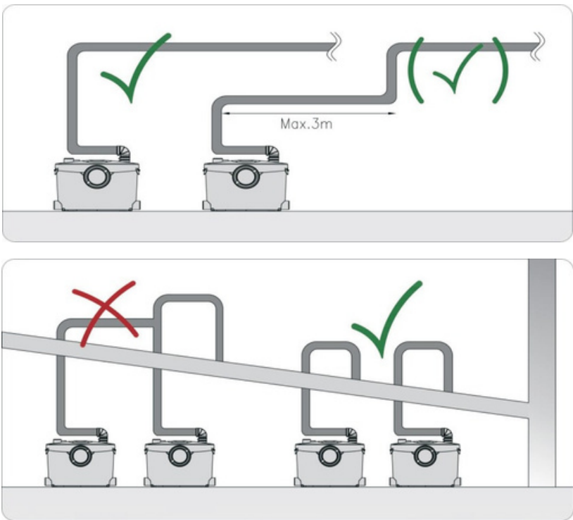
Fig14&15: Discharge pipe connection
