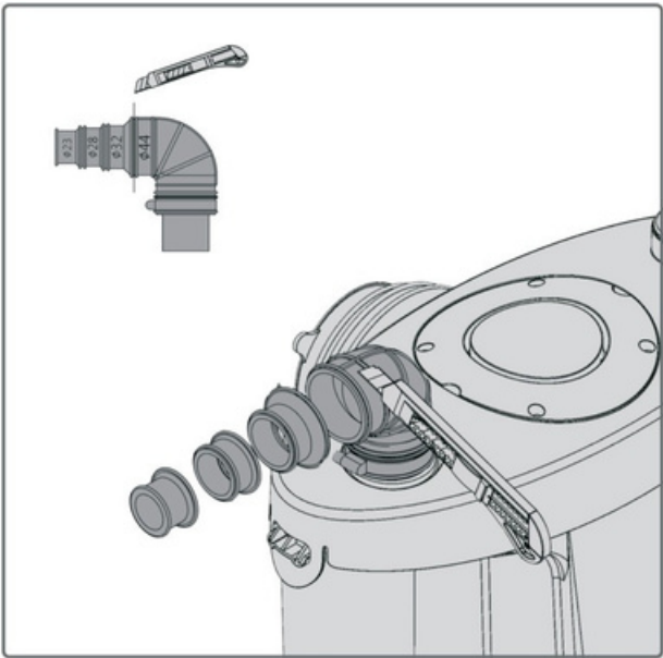
Fig8: Outlet (Check Valve)
