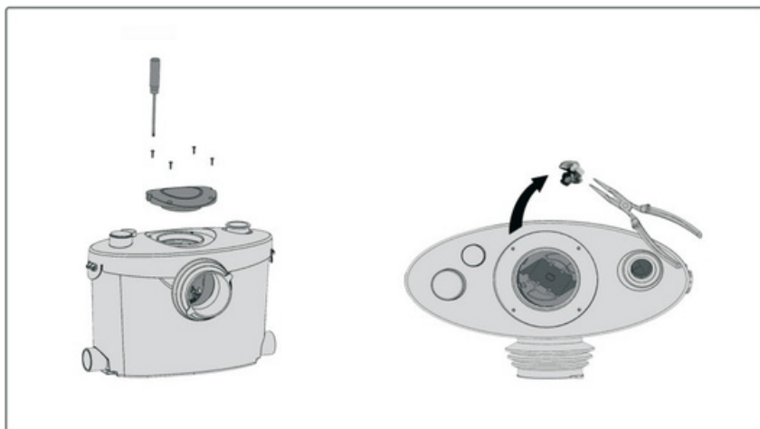
Fig10: Pumping head
