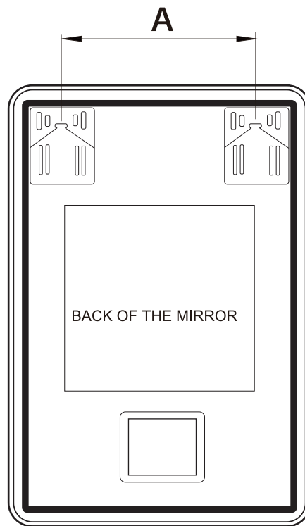
Vertical Mounting
